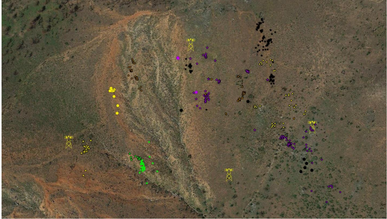
Figure 12. Verified queer source locations at the chaparral study site, May 5 th and 9 th , 2016. Colors indicate different individuals identified by unique voice sonograms. Different shapes indicate morning versus evening calling periods among individuals. Yellow towers indicate ARU locations.
